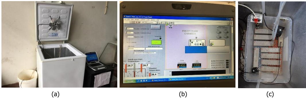
Fig. 2 | Mortar freeze and thaw test: (a) global equipment, (b) developed software and (c) recipient with tested samples with pump, water agitator, heater and temperature sensors
