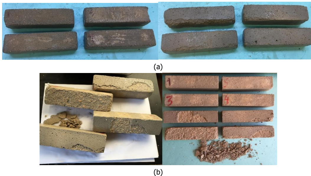
Fig. 6 | Visual aspect after freeze and thaw cycles; (a) veneer mortar; (b) infill mortar
