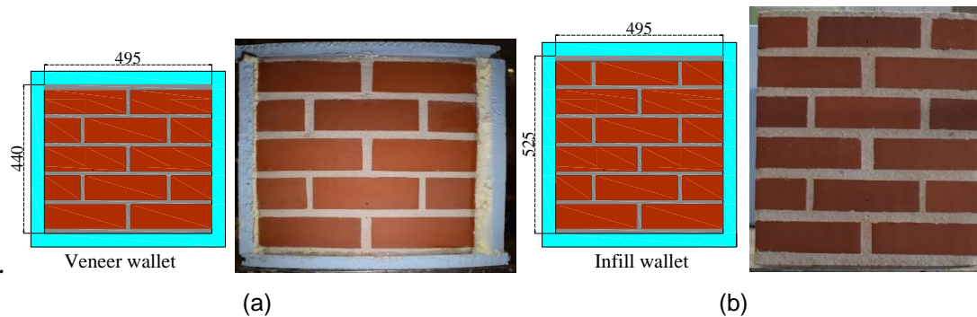
Fig. 1 | Tested masonry wallets using (a) veneer and (b) infill mortar (dimensions in mm)
